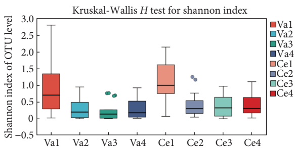
图 3 不同时间点阴道及宫颈微生物Shannon指数比较箱形图 Fig 3 Boxplot of the Shannon index of vaginal and cervical microorganisms at different time points
