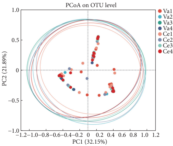
图 4 不同时间点阴道及宫颈微生物主成分分析 Fig 4 Principal Component Analysis of vaginal and cervical microorganisms at different time points
